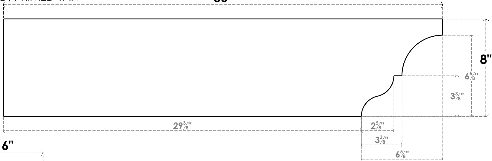
SIDE PROFILE
